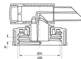
Screwcap
